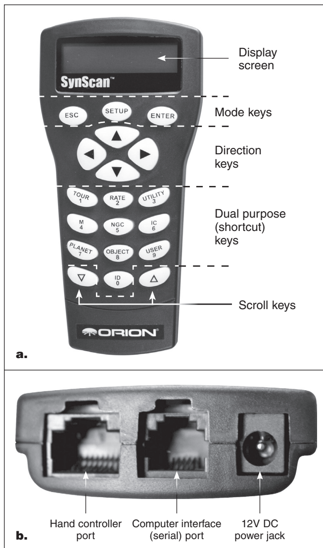
Figure 1. a) The SynScan GoTo hand controller. b) Connection ports on bottom of controller.
