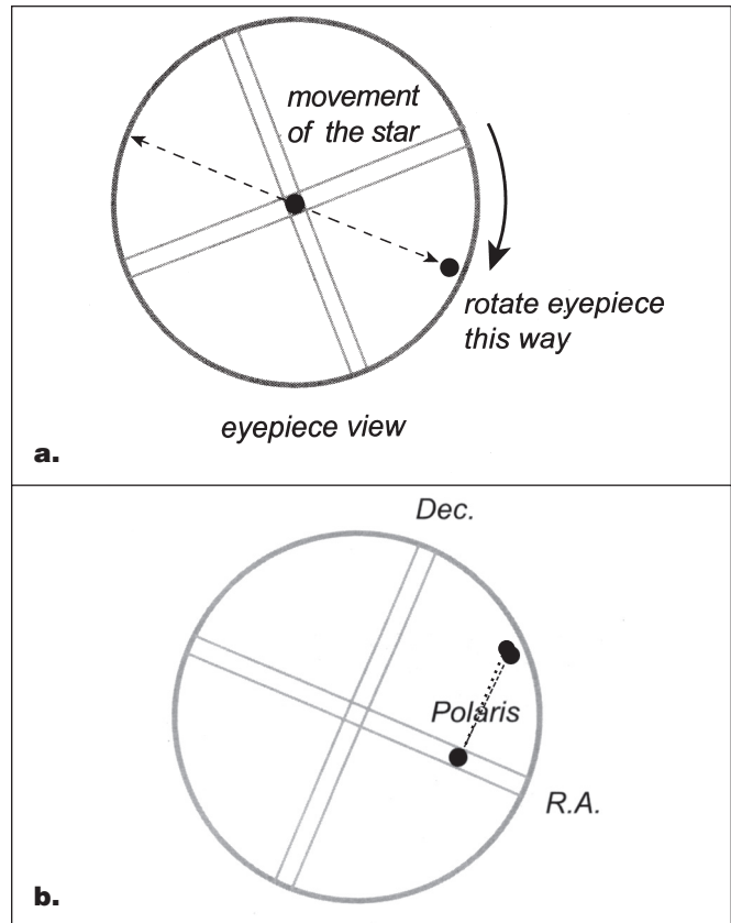
Figure 5. a) Aligning the R.A. motion of the star with the crosshairs of a reticle eyepiece. b) Adjust the telescope in Dec. (with the hand controller) to place the star on the R.A. crosshair.
